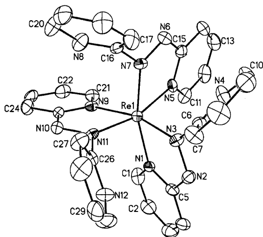
Figure 1. Perspective view and atom labeling scheme of [\text{ReL}_3]^+ ; all non-hydrogen atoms are represented by 30% thermal probability ellipsoids (hydrogen atoms are omitted for clarity); selected bond lengths [Å]: Re1–N3 1.965(9), Re1–N7 1.999(9), Re1–N5 2.111(8), Re1–N11 1.982(7), Re1–N1 2.110(8), Re1–N9 2.115(8), N2–N3 1.360(12), N10–N11 1.333(10), N6–N7 1.312(11); selected bond angles [°]: N3–Re1–N11 96.1(3), N11–Re1–N7 96.0(3), N11–Re1–N1 97.0(3), N3–Re1–N5 96.7(3), N7–Re1–N5 73.4(4), N3–Re1–N9 164.9(3), N7–Re1–N9 97.1(3), N5–Re1–N9 95.3(3), N3–Re1–N7 95.1(4), N3–Re1–N1 74.5(3), N7–Re1–N1 164.1(3), N11–Re1–N5 164.0(3), N1–Re1–N5 95.5(3), N11–Re1–N9 73.8(3), N1–Re1–N9 95.2(3)
