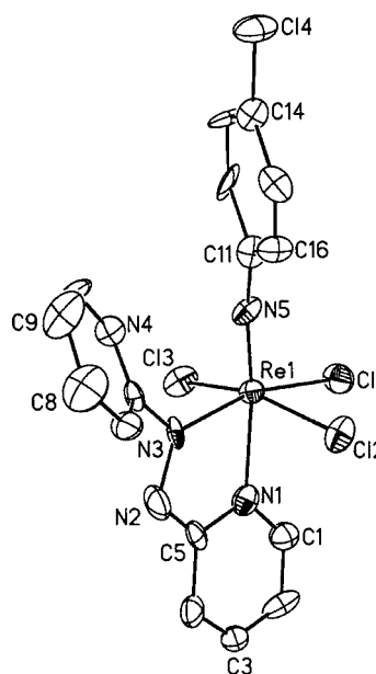
Figure 3. Perspective view and atom labeling scheme of [\text{ReCl}_3(\text{NC}_6\text{H}_4\text{Cl-}p)\text{L}] ; all non-hydrogen atoms are represented by 30% thermal probability ellipsoids (hydrogen atoms are omitted for clarity) selected bond lengths [Å]: Re1–N5 1.72(2), Re1–N1 2.18(3), Re1–N3 2.00(2), Re1–Cl1 2.354(9), Re1–Cl2 2.386(9), Re1–Cl3 2.335(9), N2–N3 1.30(4)
