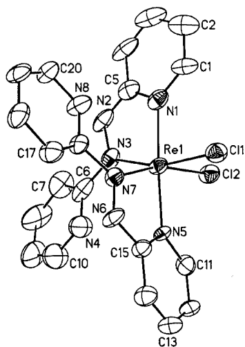
Figure 2. Perspective view and atom labeling scheme of [\text{ReL}_2\text{Cl}_2] ; all non-hydrogen atoms are represented by 30% thermal probability ellipsoids (hydrogen atoms are omitted for clarity); selected bond lengths [Å]: Re1–N3 2.001(13), Re1–N5 2.043(10), Re1–N7 2.005(11), Re1–N1 2.080(13), Re1–Cl2 2.374(4), Re1–Cl1 2.384(4), N2–N3 1.37(2), N6–N7 1.32(2); selected bond angles [°]: N3–Re1–N7 91.8(5), N7–Re1–N5 74.4(4), N7–Re1–N1 108.3(5), N3–Re1–Cl2 93.4(4), N5–Re1–Cl2 90.3(3), N3–Re1–Cl1 163.4(4), N5–Re1–Cl1 88.6(3), Cl2–Re1–Cl1 92.25(14), N3–Re1–N5 106.9(5), N3–Re1–N1 75.0(6), N5–Re1–N1 176.8(4), N7–Re1–Cl2 164.7(3), N1–Re1–Cl2 87.0(3), N7–Re1–Cl1 86.8(4), N1–Re1–Cl1 89.7(4)
